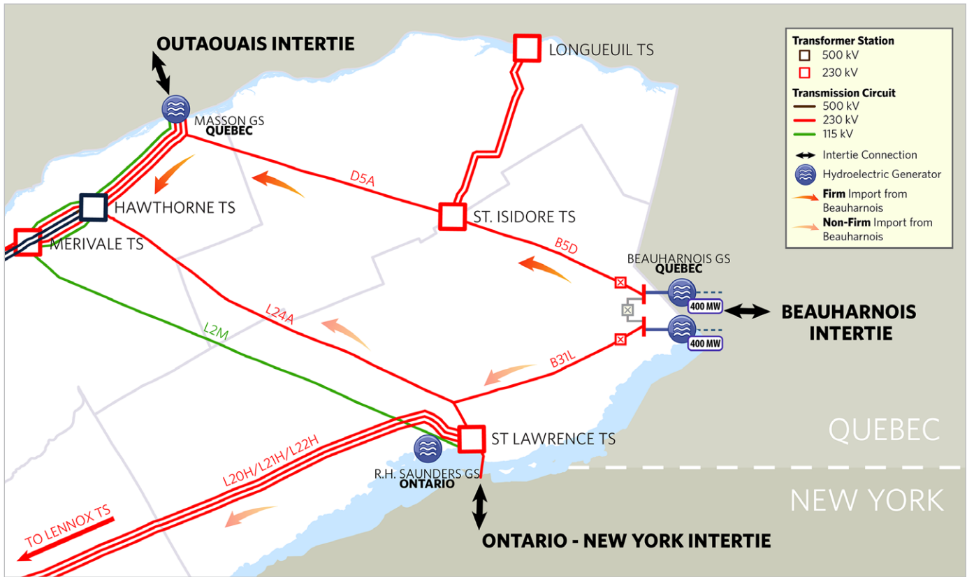
Figure 8. 230 kV Circuits between Hawthorne TS and Merivale TS
