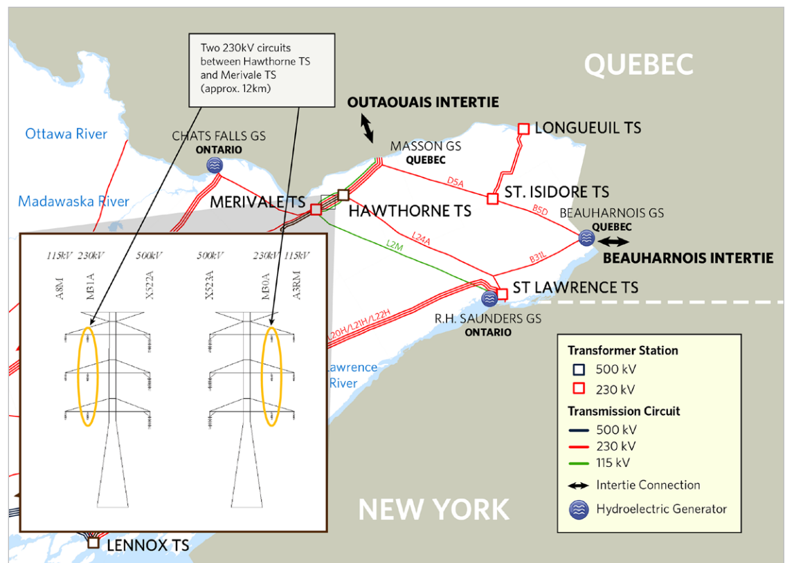
Figure 7. 230 kV Circuits between Hawthorne TS and Merivale TS
