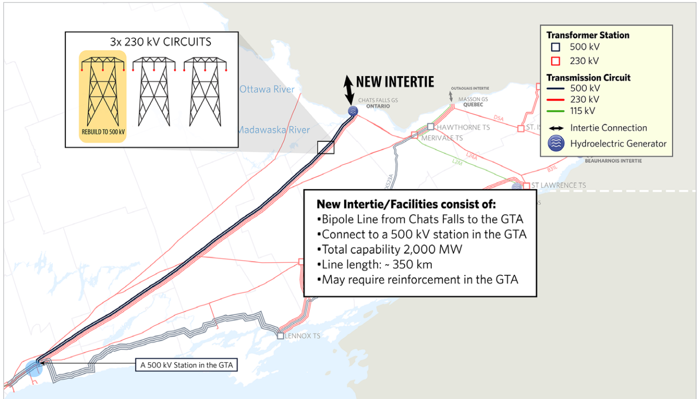
Figure 12. New Intertie at Chats Falls
