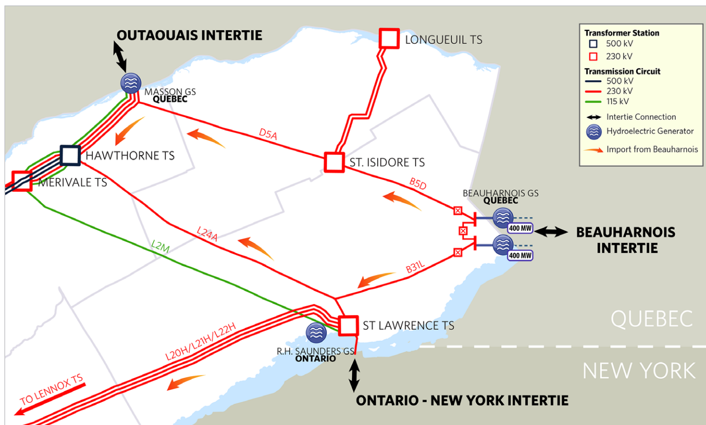
Figure 6. St. Lawrence TS Hub and the Transmission System in South Eastern Ontario
