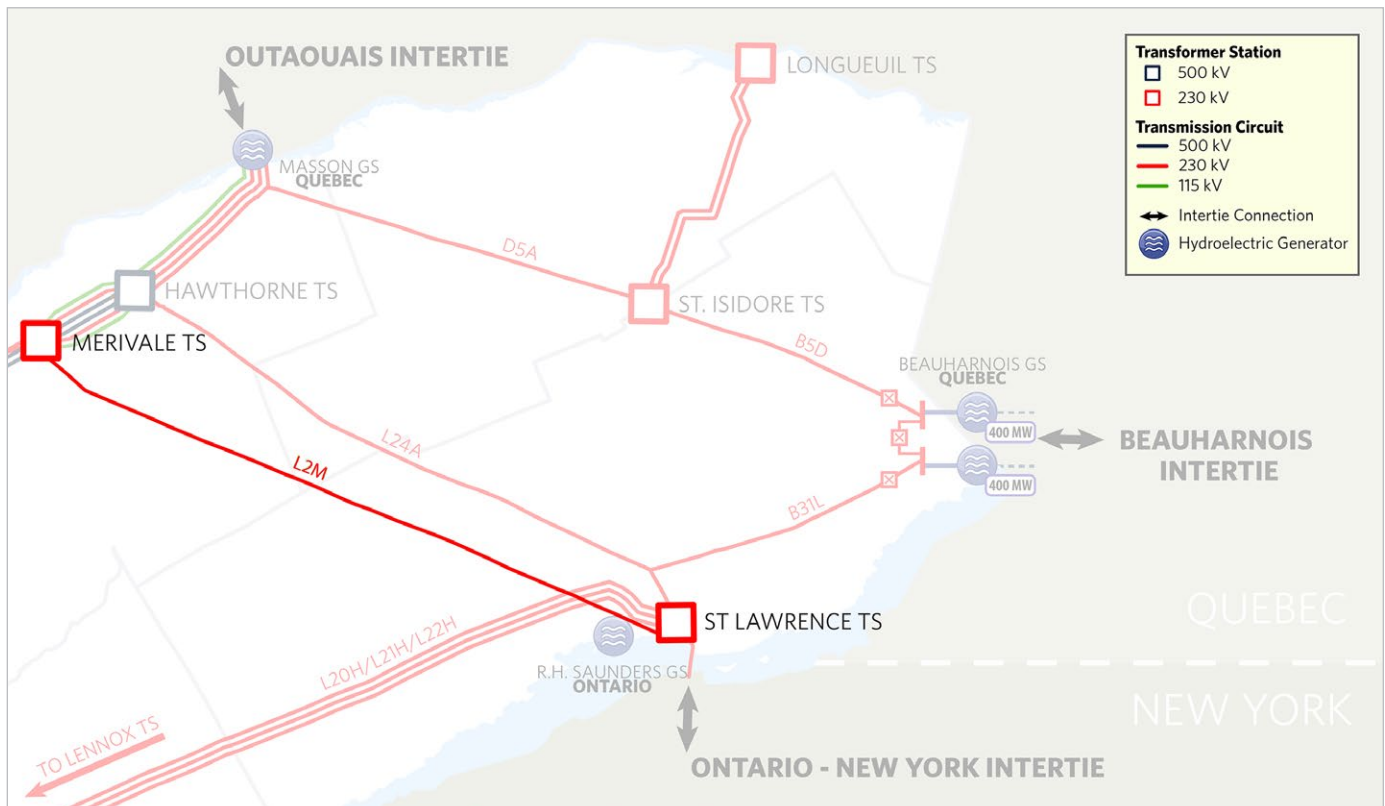
Figure 9. Rebuild Existing 115 kV circuit L2M to be a Double- Circuit 230 kV Transmission Line
