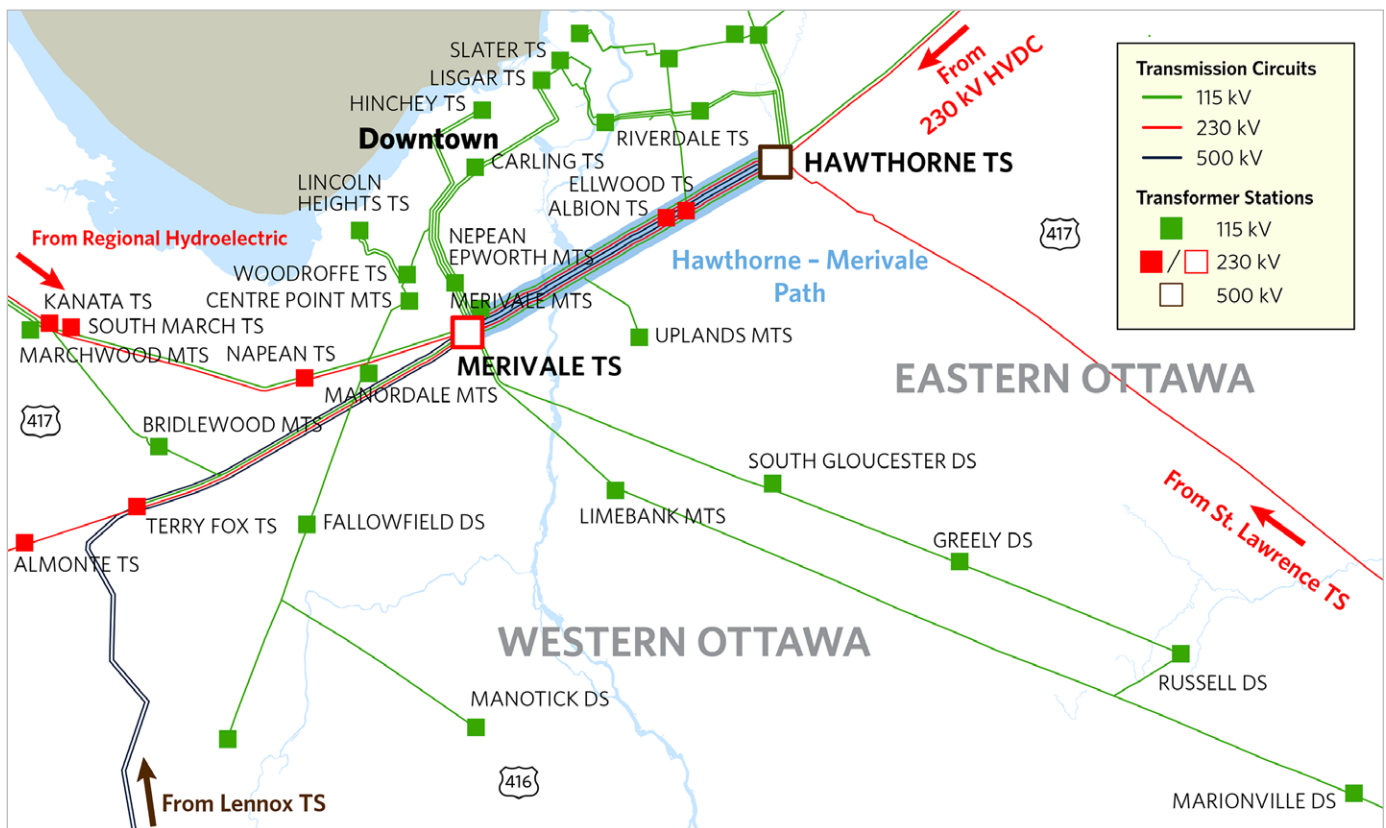
Figure 5. Hawthorne TS Hub and the Transmission System in the Ottawa Area
