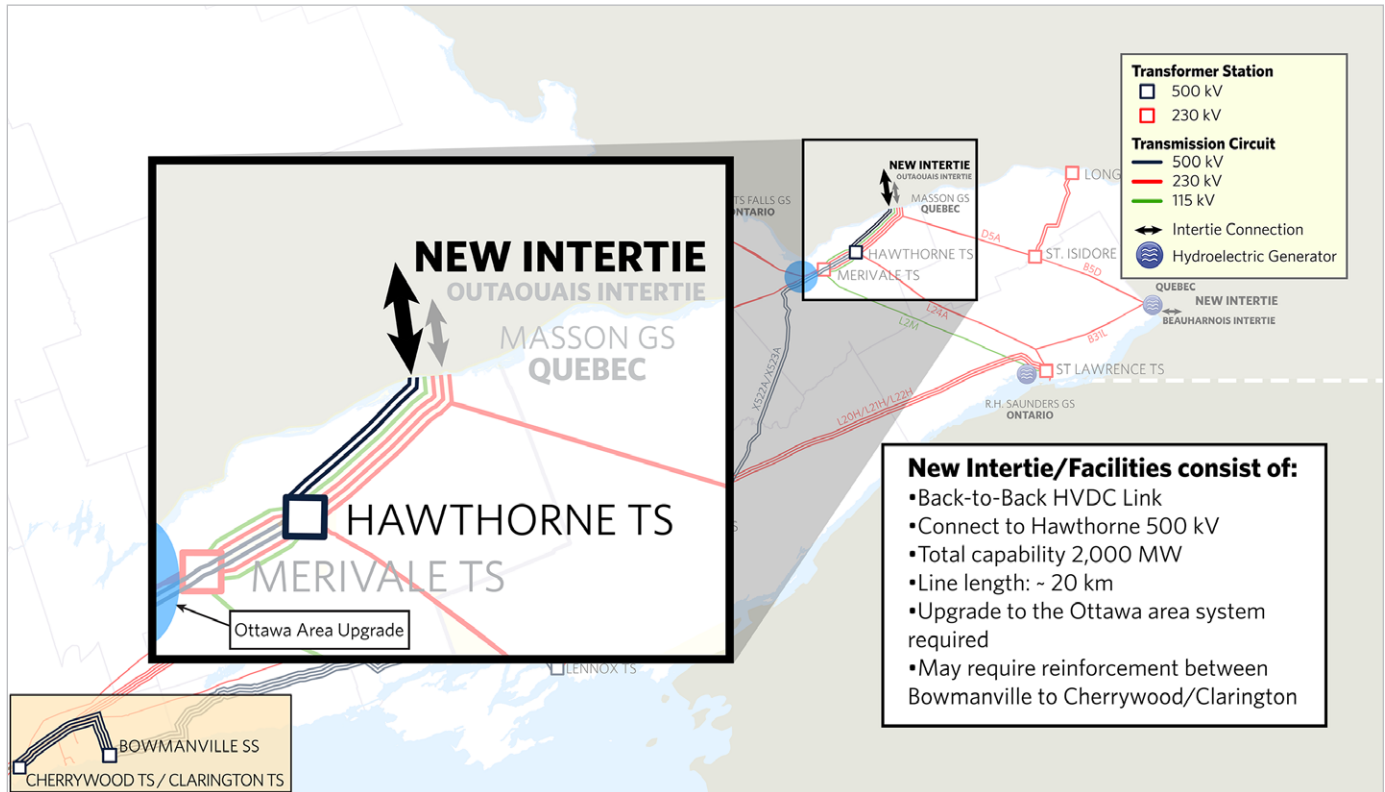
Figure 10. New Intertie at Outaouais
