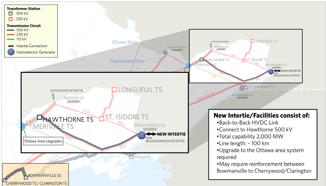
Figure 11. New Intertie at Beauharnois
