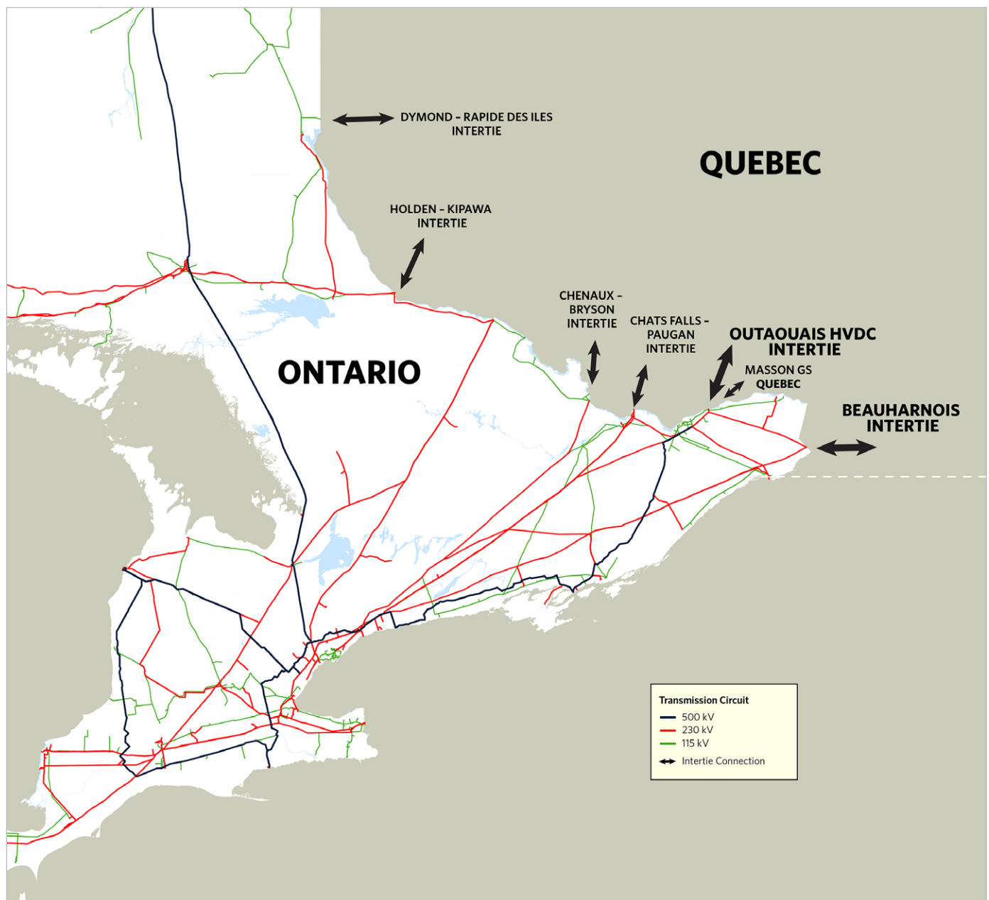
Figure 1. Existing Ontario-Quebec Interconnections
