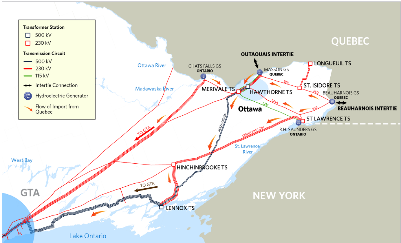
Figure 4. Eastern Ontario Transmission Network
